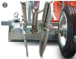
Striping unit with limiter discs, line width adjustable
